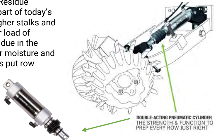
Figure 1. CleanSweep® System
