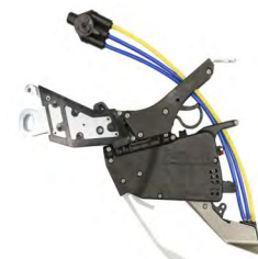
Figures 2-3: FurrowJet® Dual-Band Wings Fracturing Sidewalls
