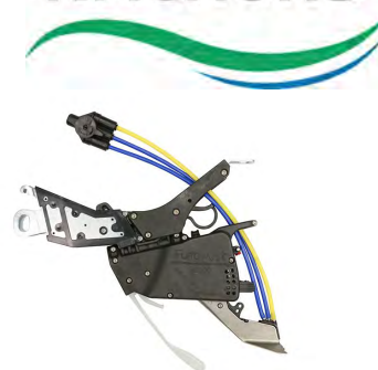
Figure 1. FurrowJet® Placement
