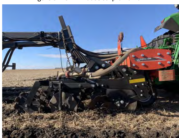
Figure 3. KUHN Krause strip-till unit
